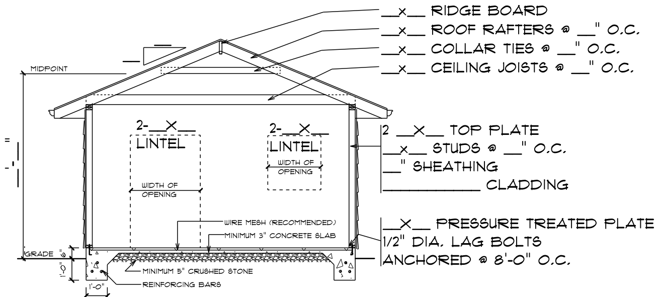
FLOATING SLAB (MAX 538 SQ.FT.)
