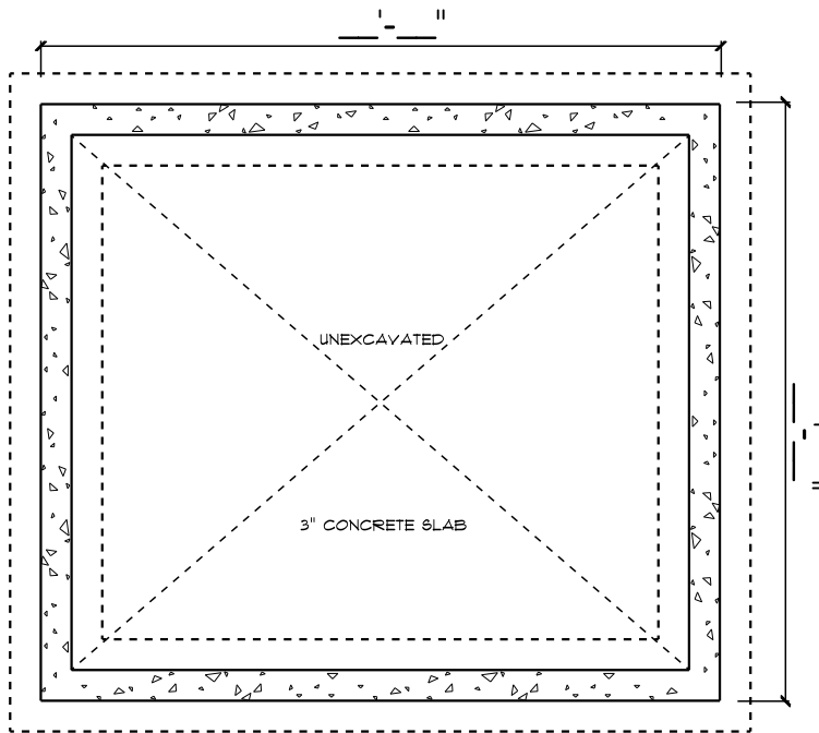
FROST FOOTING PLAN
