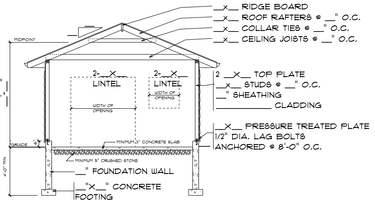
CROSS SECTION
