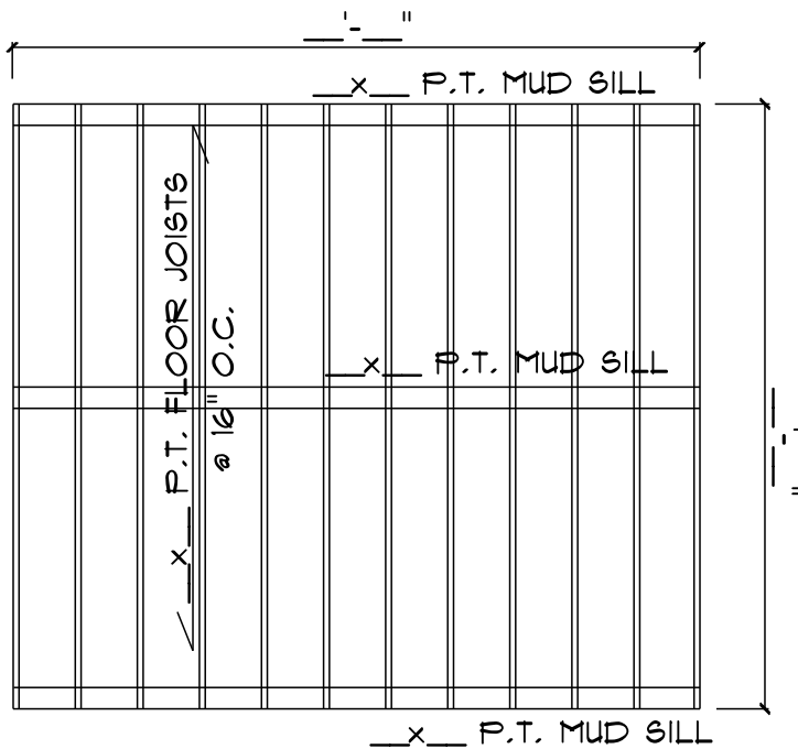
MUD SILL PLAN
