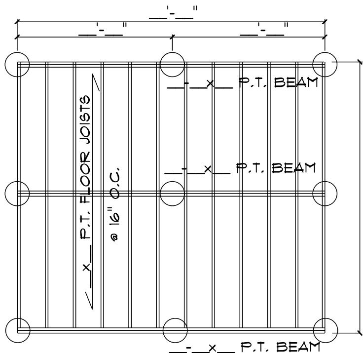
PIER FOOTING PLAN
